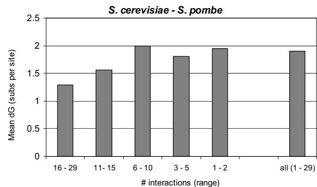
Figure 2 Mean evolutionary rates between S. cerevisiae and S. pombe orthologs for bins of proteins with different numbers of interactions. The range of the number protein-protein interactions per S. cerevisiae protein for each bin (x-axis) and the mean evolutionary rate (substitutions per site) for each bin (y-axis).
