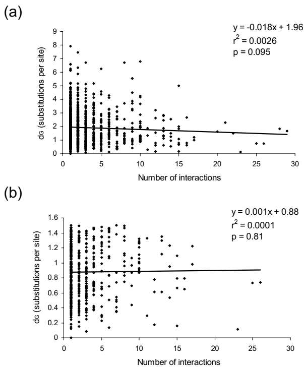
Figure 1 The relationship between the number of protein-protein interactions for S. cerevisiae proteins and the evolutionary rates between S. cerevisiae and S. pombe orthologs. Shown for each plot is the equation that describes the linear trend line, the r^2 value that describes the fraction of the variability in the evolutionary rates that is accounted for by the variability in the number of protein-protein interactions and the p value, which is the probability that the correlation between the number of protein-protein interactions and evolutionary rates could be due to chance. (a) All 1,061 observations. (b) 478 observations that correspond to orthologous protein pairs with = 40% amino acid sequence identity.
